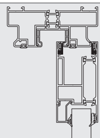
PVC16 - PVC DESTEK PARÇASI / 100 mm PVC16 - PVC SUPPORT PART / 100 mm
