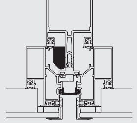
PVC12 - TAKOZ / 100 mm PVC12 - SUPPORT PART / 100 mm
