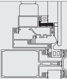
PVC11 - CAM TAKOZU / 100 mm PVC11 - GLASS WEDGE / 100 mm
