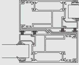
KLF01 - KIL FİTİL / 6 mm KLF01 - WEATHER STRIP / 6 mm
