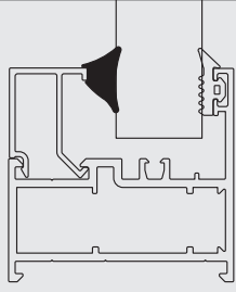
FTL04 - İÇ CAM FİTİLİ / 105 gr FTL04 - GLAZING GASKET INSIDE / 105 gr
