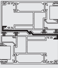
PVC15 - KENET PVC PROFİLİ / 6000 mm PVC15 - PVC PROFILE / 6000 mm
