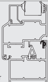
FTL06 - BİNİ FİTİLİ / 30 gr FTL06 - ACOUSTICAL GASKET OUTSIDE / 30 gr
