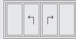
HEBESCHIEBE AKSESUARI - C TİPİ LIFT and SLIDE MECHANISM TYPE C
