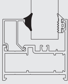
FTL02 - İÇ CAM FİTİLİ / 80 gr FTL02 - GLAZING GASKET INSIDE / 80 gr
