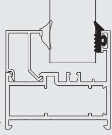
FTL07 - DİŞ CAM FİTİLİ / 70 gr FTL07 - GLAZING GASKET OUTSIDE / 70 gr
