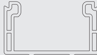
PVC14 - KASA İÇİ PVC PROFİL / 6000 mm PVC14 - PVC PROFILE FOR FRAME / 6000 mm
