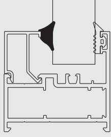
FTL03 - İÇ CAM FİTİLİ / 90 gr FTL03 - GLAZING GASKET INSIDE / 90 gr
