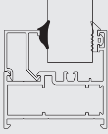
FTL01 - İÇ CAM FİTİLİ / 65 gr FTL01 - GLAZING GASKET INSIDE / 65 gr
