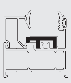
PVC01 - CAM TAKOZU / 100 mm PVC01 - GLASS WEDGE / 100 mm
