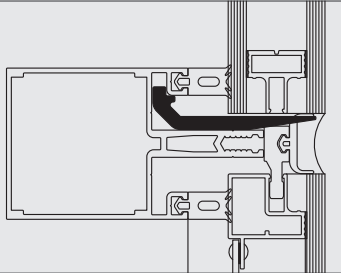
HLD01 / CAM TAKOZU 100 mm HLD01 / GLASS WEDGE 100 mm
