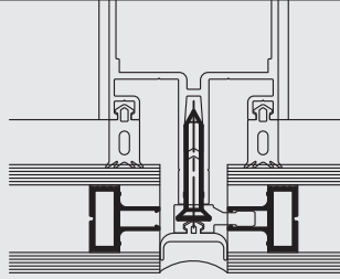
NA01 - CAM ARA PROFİLİ NA01 - GLASS ADAPTER PROFILE
