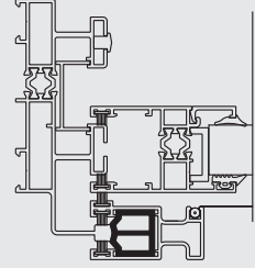
FTL41 - ÇARPMA FİTİLİ / ADET FTL41 - STOPPER GASKET / PIECE
