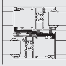
PVC06 - KENET PVC PROFİLİ / 6000 mm PVC06 - PVC Adapter Profile / 6000 mm
