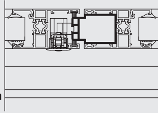
PVC08 - KENET PVC PROFİLİ / 6000 mm PVC08 - PVC Adapter Profile / 6000 mm
