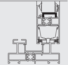
PVC04 - CAM TAKOZU / 100 mm PVC04 - GLASS WEDGE / 100 mm
