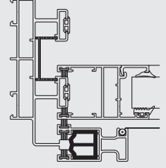
FTL41 - ÇARPMA FİTİLİ / ADET FTL41 - STOPPER GASKET / PIECE
