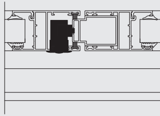
HKL01 - HAVUZ KOL TAKIMI HKL01 - COUPLING KIT
