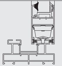
FTL03 - İÇ CAM FİTİLİ / 90 gr FTL03 - GLAZING GASKET INSIDE / 90 gr
