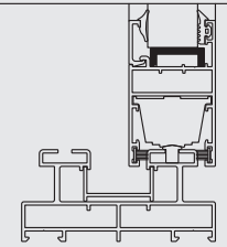
PVC04 - CAM TAKOZU / 100 mm PVC04 - GLASS WEDGE / 100 mm
