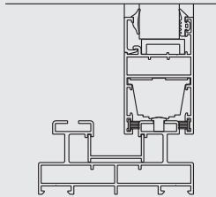
KLF01 - KİL FİTİL / 6 mm KLF01 - WEATHER STRIP / 6 mm
