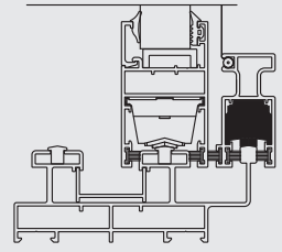
RLM02 - SİNEKLİK RULMANI RLM02 - PULLEY FOR FLYING SCREEN
