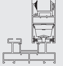
FTL01 - İÇ CAM FİTİLİ / 65 gr FTL01 - GLAZING GASKET INSIDE / 65 gr
