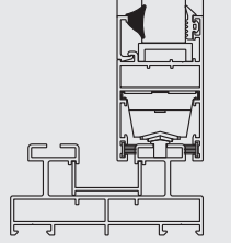
FTL04 - İÇ CAM FİTİLİ / 105 gr FTL04 - GLAZING GASKET INSIDE / 105 gr
