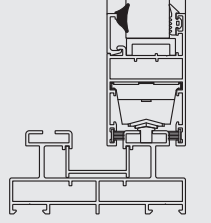
FTL02 - İÇ CAM FİTİLİ / 80 gr FTL02 - GLAZING GASKET INSIDE / 80 gr
