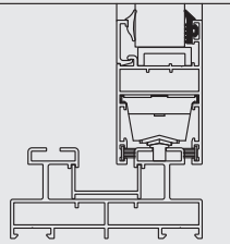
FTL07 - DIŞ CAM FİTİLİ / 70 gr FTL07 - GLAZING GASKET OUTSIDE / 70 gr
