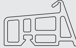
FTL37 - TOZLUK FİTİLİ / 275 gr FTL37 - SEALING GASKET / 275 gr
