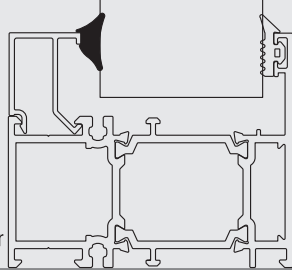
FTL02 - İÇ CAM FİTİLİ / 80 gr FTL02 - GLAZING GASKET INSIDE / 80 gr
