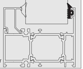
FTL07 - DİŞ CAM FİTİLİ / 70 gr FTL07 - GLAZING GASKET OUTSIDE / 70 gr
