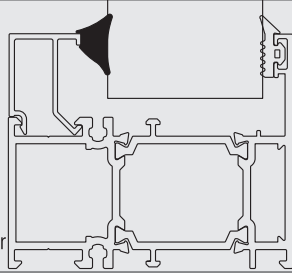
FTL04 - İÇ CAM FİTİLİ / 105 gr FTL04 - GLAZING GASKET INSIDE / 105 gr
