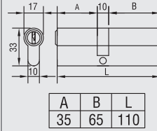
SLR02 - SİLİNDİR (110'LUK) SLR02 - CYLINDER (110)
