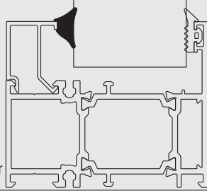
FTL03 - İÇ CAM FİTİLİ / 90 gr FTL03 - GLAZING GASKET INSIDE / 90 gr
