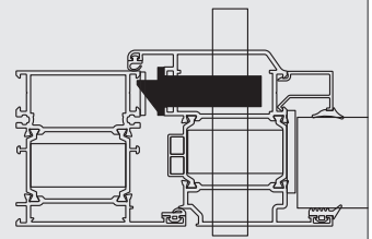
SLR02 - SİLİNDİR (110'LUK) SLR02 - CYLINDER (110)
