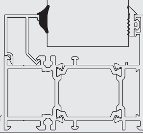
FTL01 - İÇ CAM FİTİLİ / 65 gr FTL01 - GLAZING GASKET INSIDE / 65 gr
