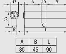
SLR01 - SİLİNDİR(90'LİK) SLR01 - CYLINDER(90)
